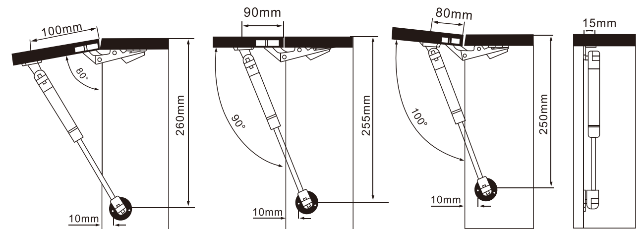
Simple installation drawing For pneumatic support
