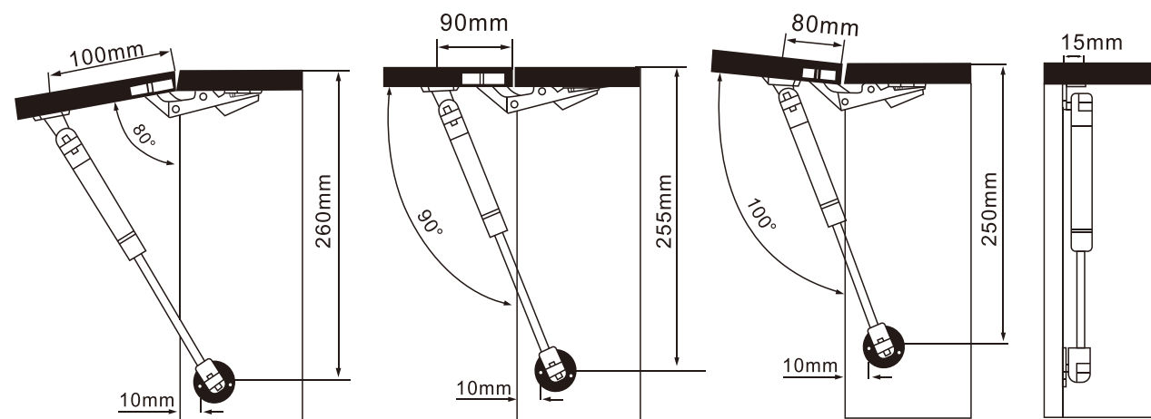
Simple installation drawing For pneumatic support
